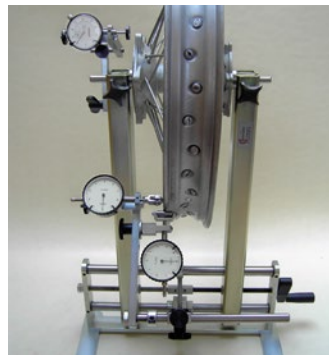
Motorbike model Screwable axle clamp · Span width 300 mm · with adapter for wheel support · Brake disc gauge as an accessory · also suitable for bicycles
